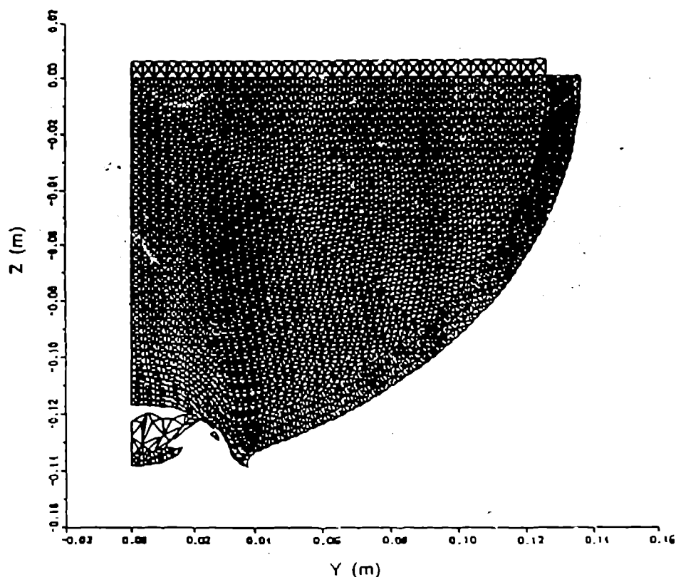
Fig. 2 - The grid at t = 20 \mu s .
