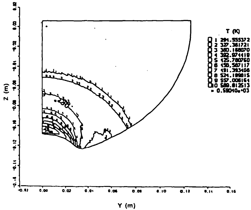
Fig. 4 - Temperature contours in the Tritonal at t = 20 \mu s for the base case.
