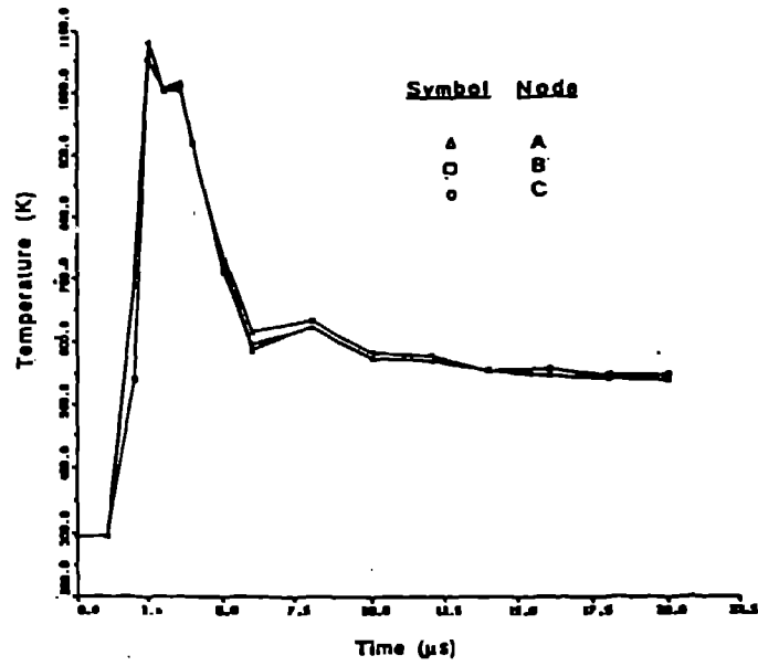
Fig. 3 - Temperature vs time profiles for the base case.
