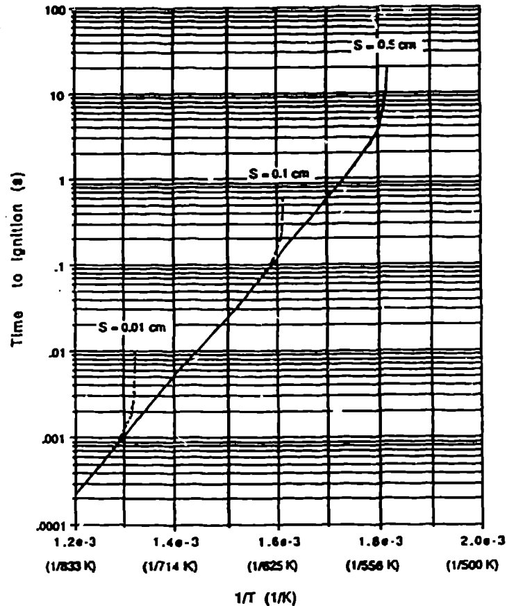
Fig. 5 - Ignition times for Tritonal slabs, low temperatures.
